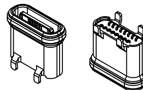
NO PART Q'TY Material 1 SHELL 1 ZINC ALLOG,NI30u"Min PLATED 2 CONTACT 16 C7025,TIN80u"/Au3u"/NI30u"PLATED 3 MID PLATE 1 SUS301,NO PLATING 4 HOUSING 1 LCP(E130i) UL94 V-0 BLACK 5 CAP 1 LCP UL94 V-0 BLACK 6 WATERPROOF RING 1 SILICONE(SI/60-65A) UL94 V-0 BLACK
